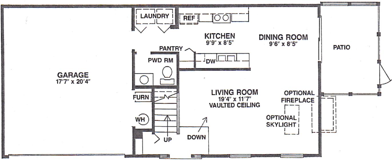
FIRST FLOOR
